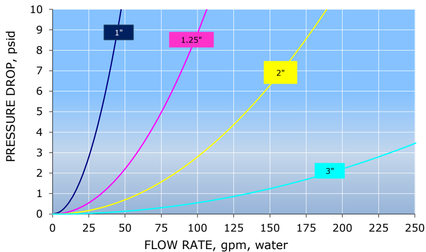
HOUSING PRESSURE DROP vs LIQUID FLOW RATE
