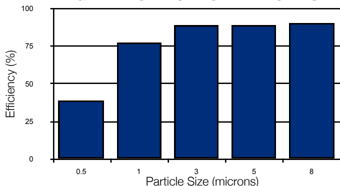
AVERAGE EFFICIENCY vs. PARTICLE SIZE
